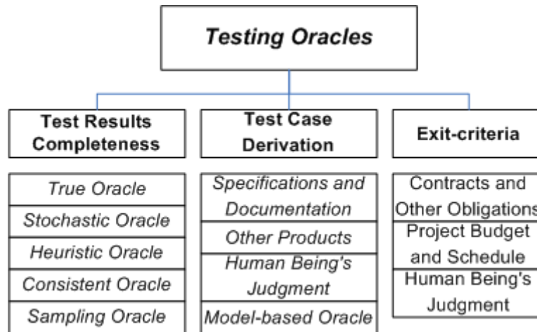
Figure 2. Testing Oracles
