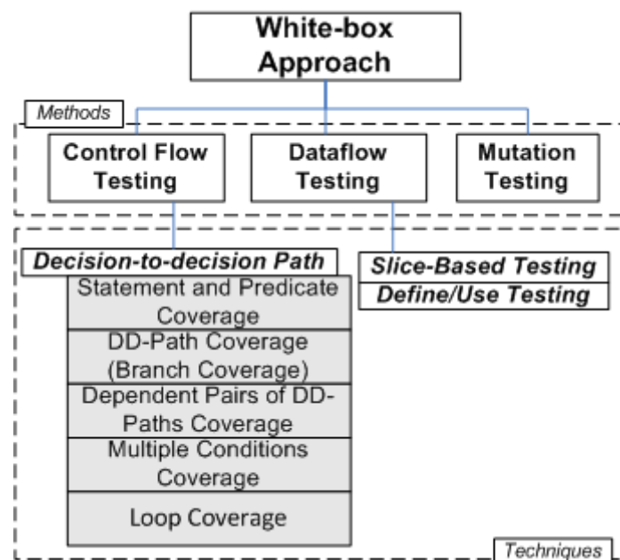
Figure 6. White-box Approach
