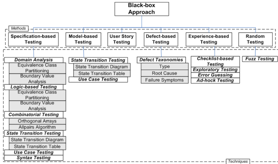
Figure 5. Black-box Approach
